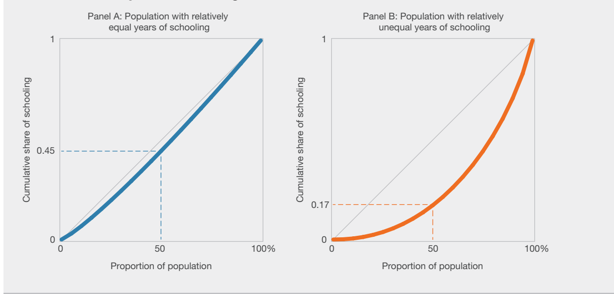
Figure 3.5 Hypothetical Lorenz curves illustrating two populations with different distributions of years of schooling
