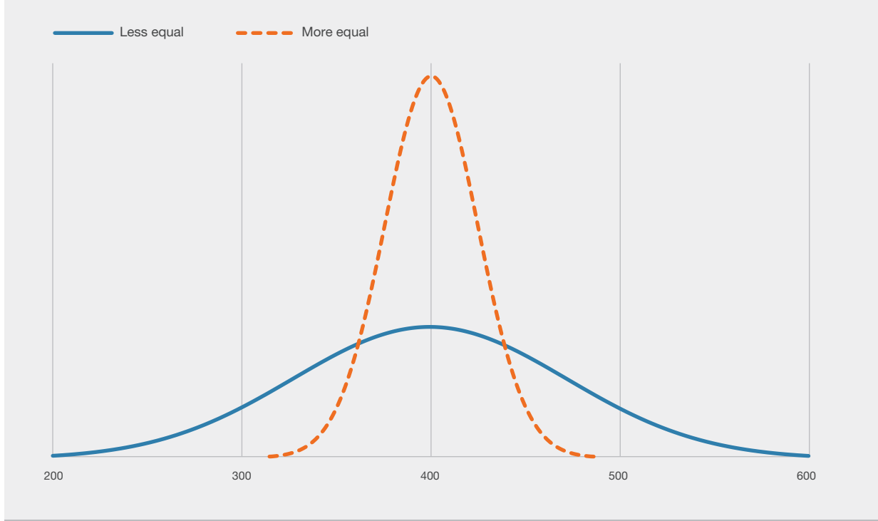
Figure 3.1 Hypothetical test score distributions with varying levels of inequality
